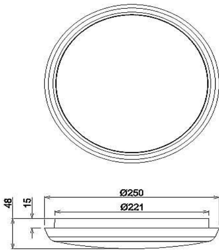
Dimensions for 250mm version
